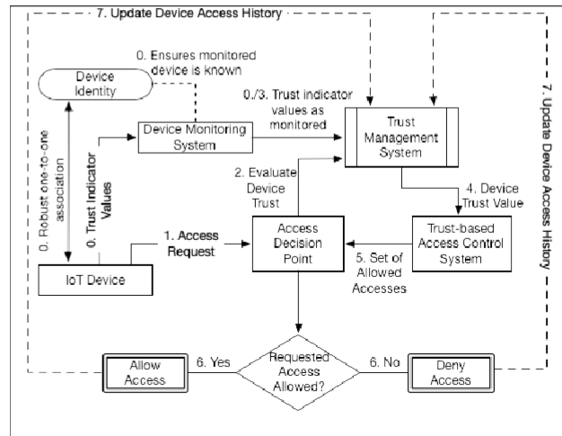
Fig. 4. IoT Trust Framework
